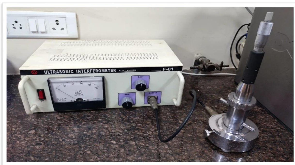
Ultrasonic Interferometer
